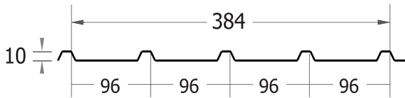
TYPE 5
