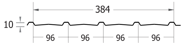
TYPE 5M
